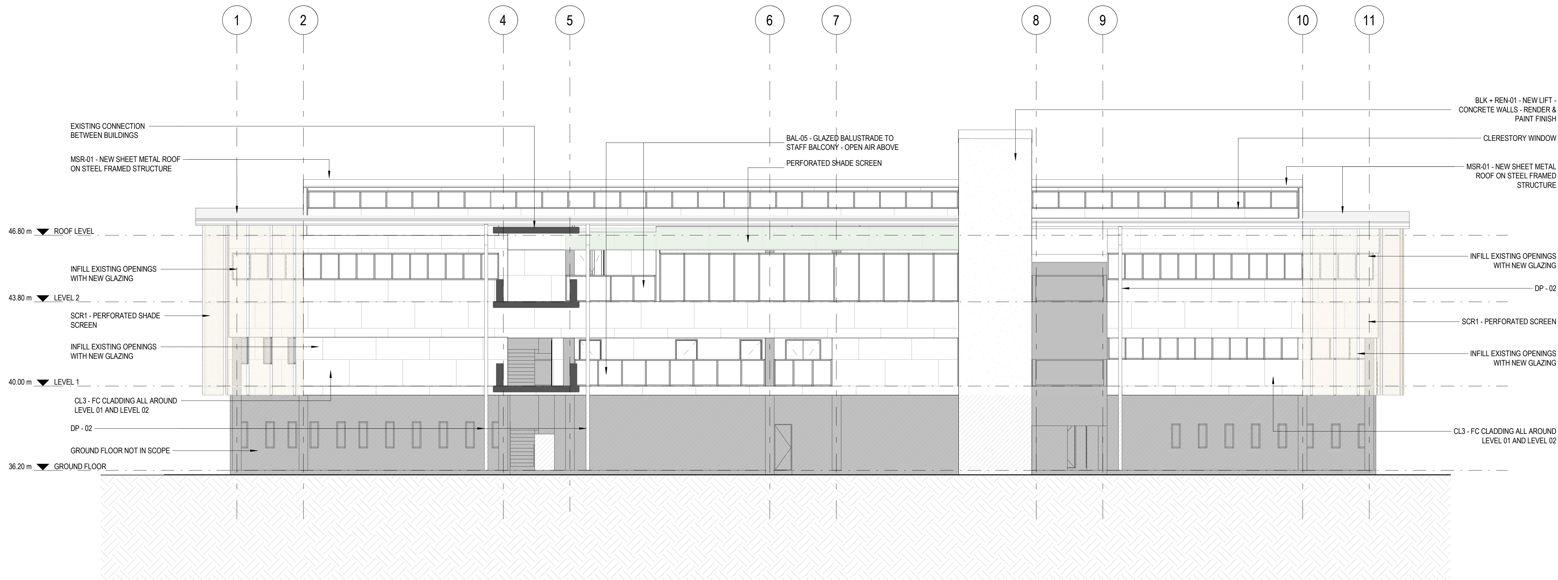
1 SOUTH ELEVATION -PROPOSED 1 : 100
